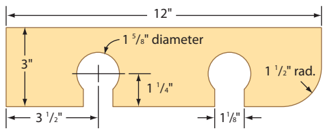
BASEBALL BAT HANGER DETAILS
