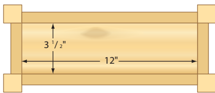
SHORT PLANTER - TOP VIEW
