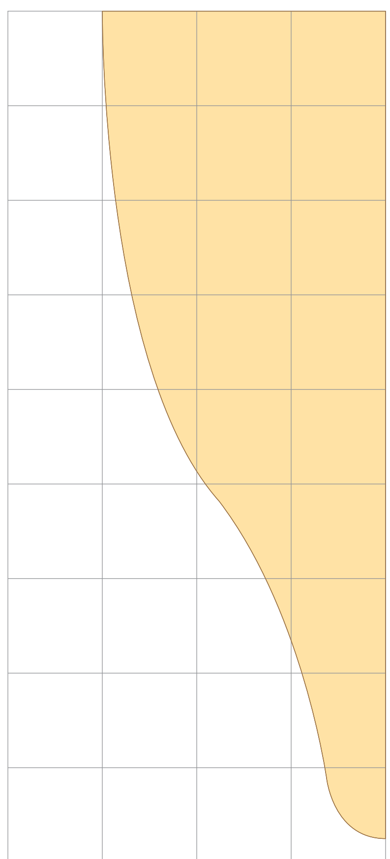
1 square = 1" ARMREST SUPPORT
