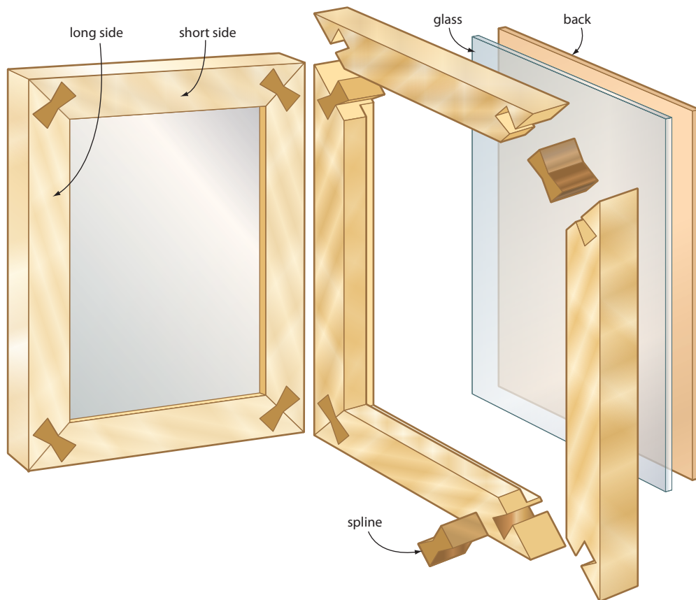
FRAME/GLASS/BACK DETAIL
