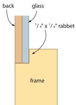
FRAME/GLASS/BACK DETAIL
