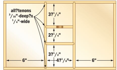
TOP TRAY TOP VIEW
