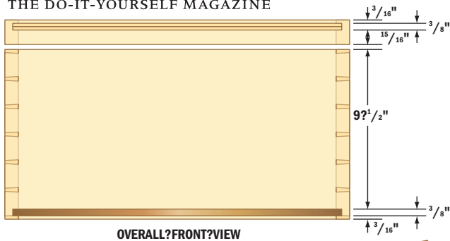
OVERALL FRONT VIEW
