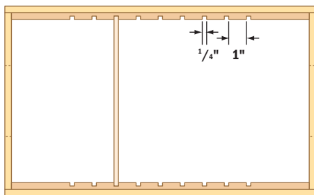
BOTTOM TRAY TOP VIEW
