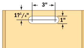
BOTTOM TRAY END VIEW
