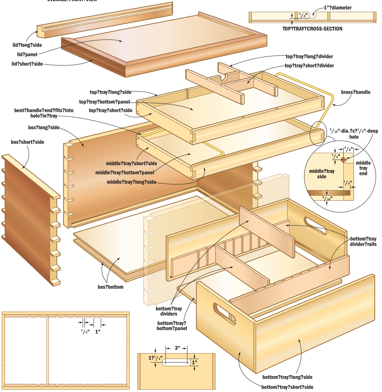
BOTTOM TRAY TOP VIEW
